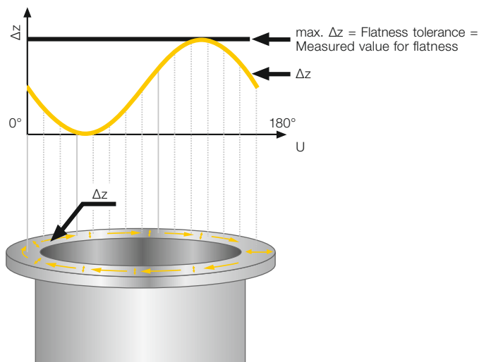
Display of double-shaft circumference imperfection
